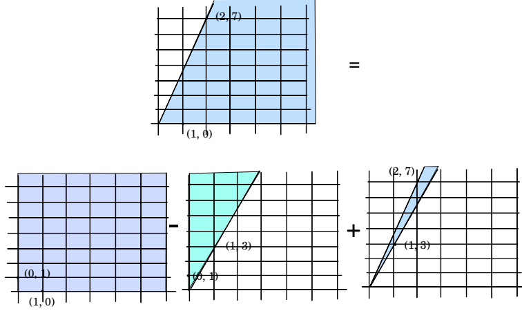
Fig. 3. Example of Barvinok's decomposition
