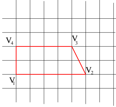
Fig. 1. A quadrilateral in Example 2.
