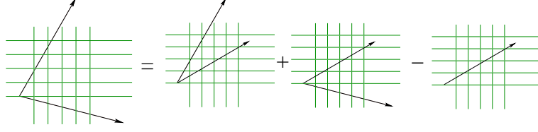
Fig. 2. Contribution of lower dimensional cones
