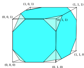
Fig. 4. The truncated cube.
