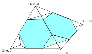
Fig. 6. The truncated simplex.
