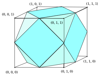
Fig. 5. The cuboctahedron.
